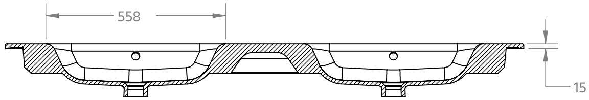
Section B-B
